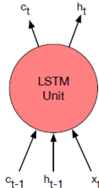
LSTM Unit
