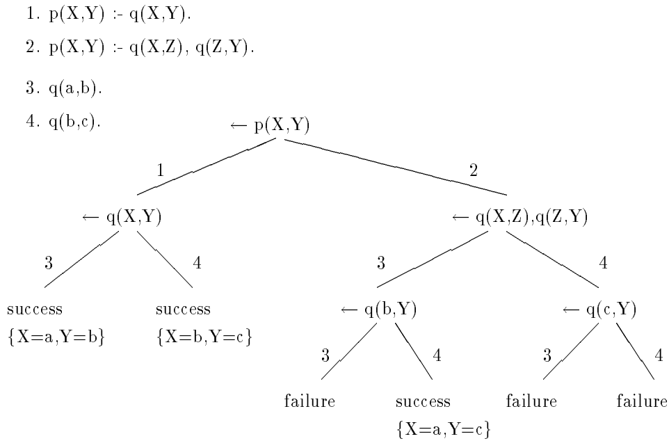
FIGURE 4.3. A Trivial Theory and Its Search Tree
