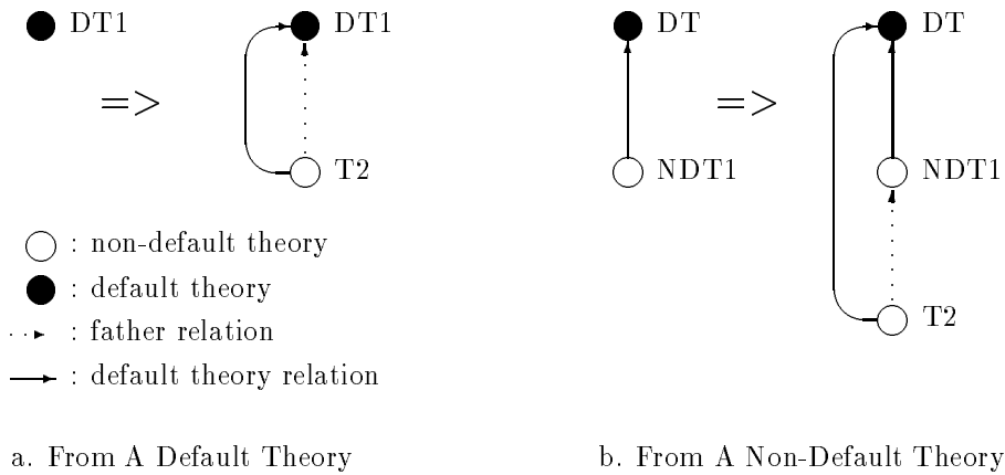
FIGURE 2.2. Creation of A Theory From Default and Non-Default Theories
