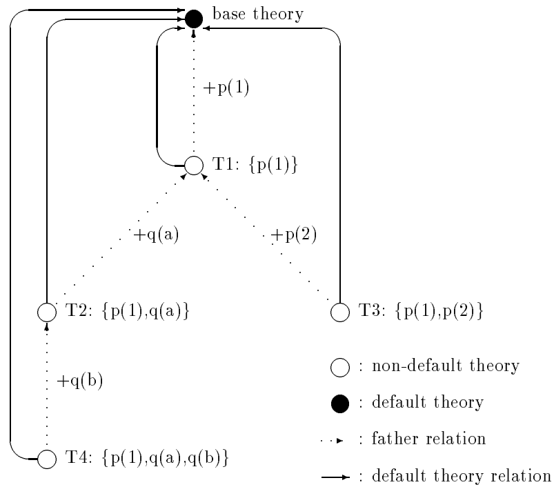
FIGURE 2.4. A Theory Tree In The Non-Default Theory Approach
