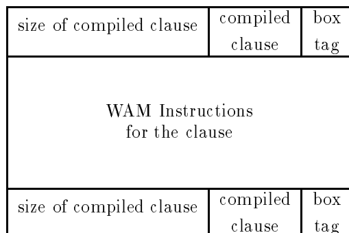
FIGURE 3.3. A Compiled Clause Box
