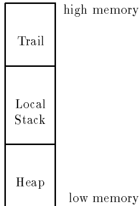
FIGURE 3.1. Memory Organization of the AMPE
