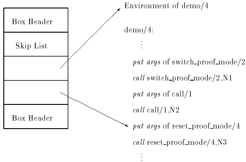
FIGURE 5.4. A Control Information Box and Demo Predicate
