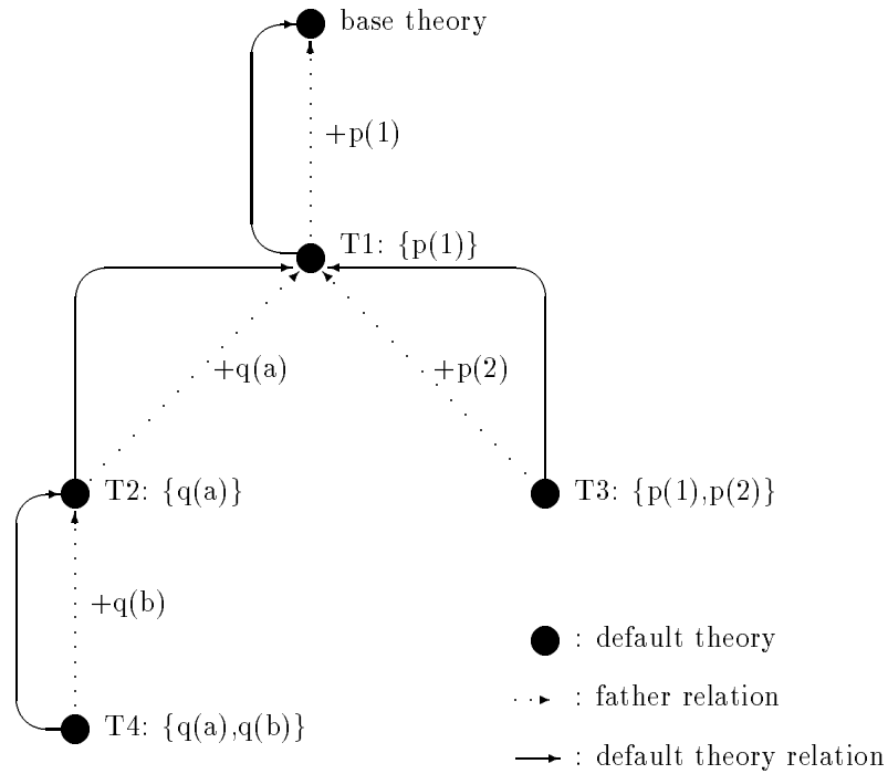
FIGURE 2.3. A Theory Tree in The Naive Approach
