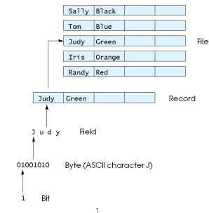
Fig. 11.1 The data hierarchy.
