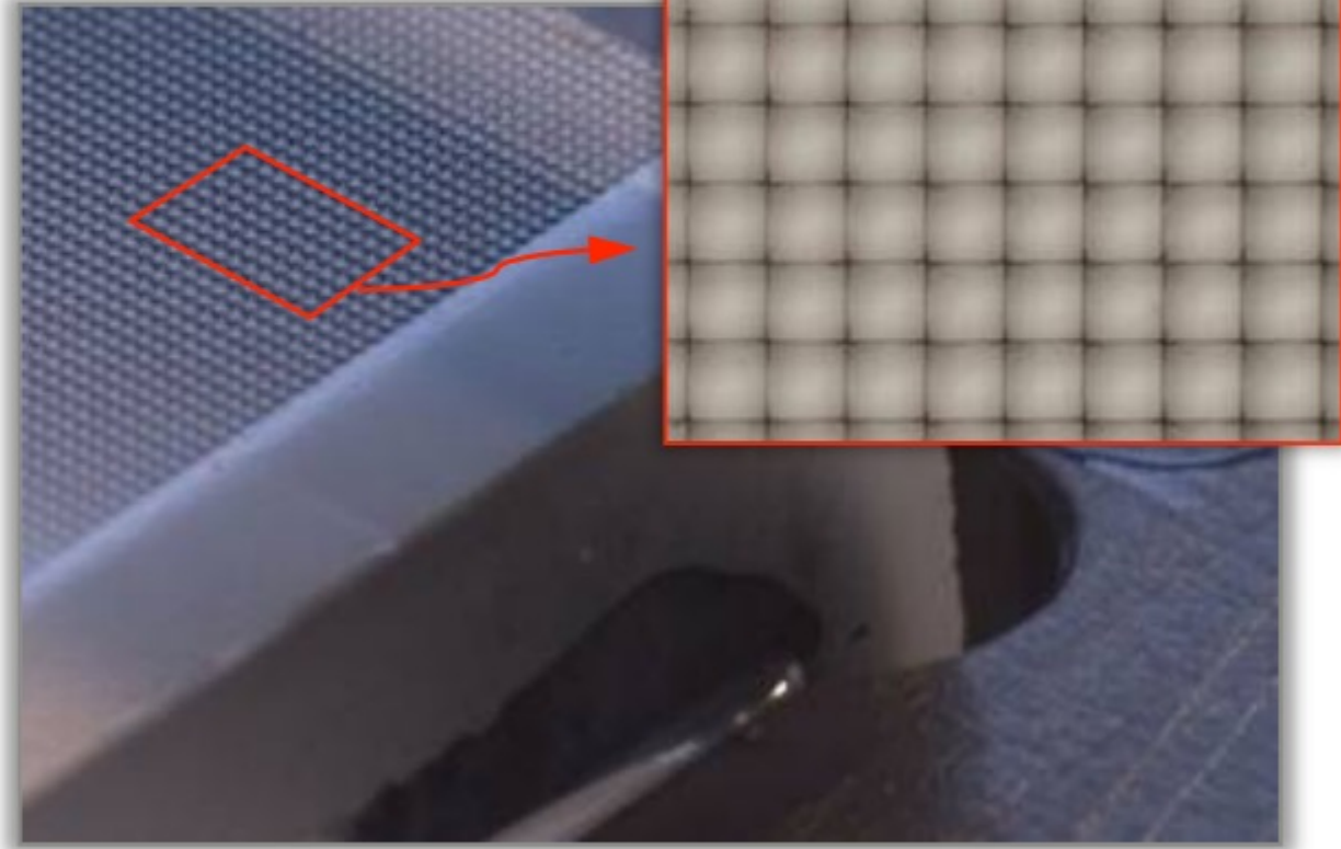
125µ square-sided microlenses
