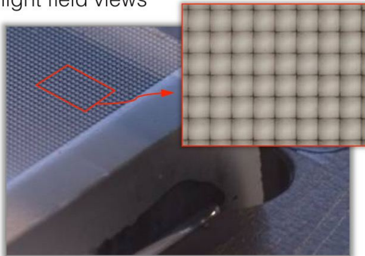
125µ square-sided microlenses
