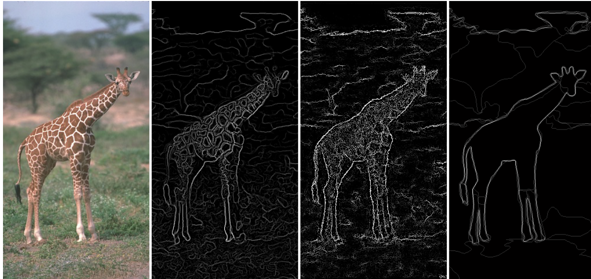
Figure 1: From left to right: (1) input image (2) boundary strength based on the average of many Canny edge detections (3) results from this project (4) average human boundary annotations. The Canny detector responds strongly to the interior texture of the giraffe instead of its boundary against the background. The Sketch Token result agrees more with human boundary annotation. The multitude of weaker boundary detections are not a problem as long as they are less confident than the correct boundaries.
