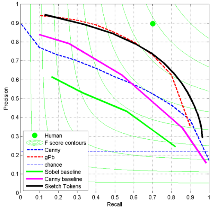
Figure 2: Dotted lines are copied from figure 17 in Arbelaez et al. 2011. Solid lines come from our implementations. Light green lines are iso-F measure lines.
