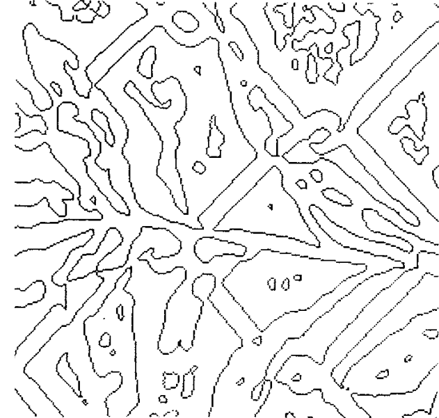
zero-crossings
