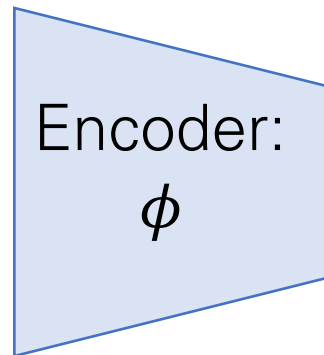
Features: \phi(x)
