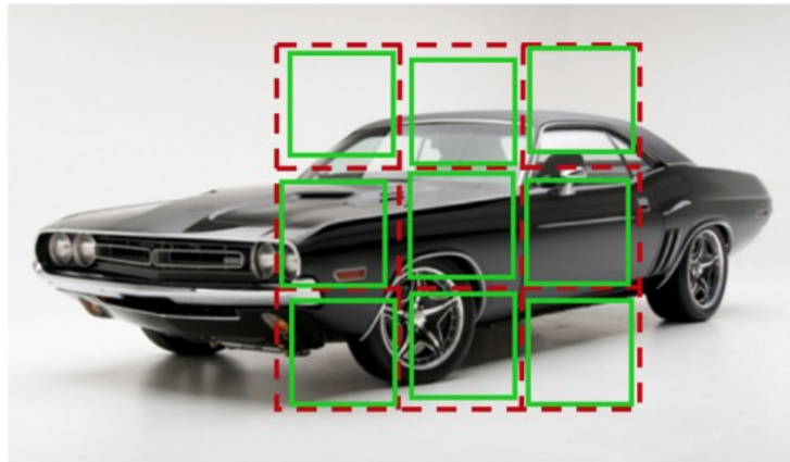
Permutation Set
