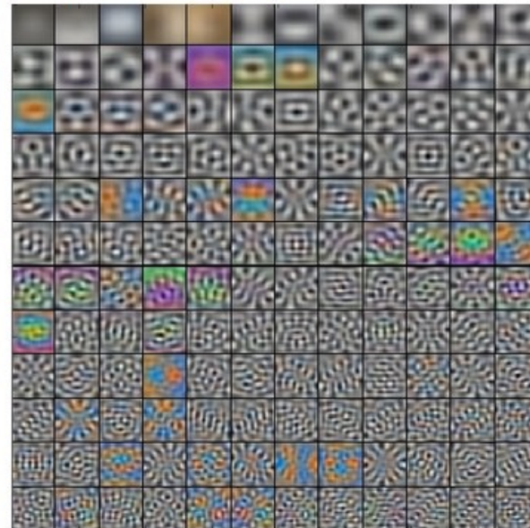
top 144 eigenvectors
