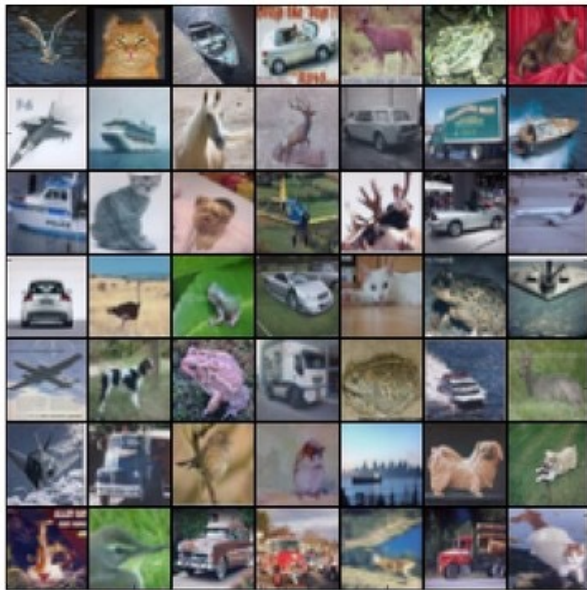
original images
