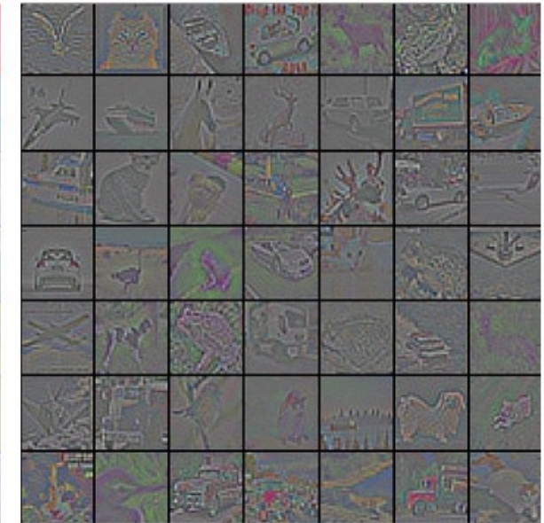
whitened images
