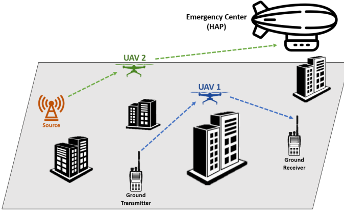
Fig. 1. System overview of the proposed DDQN-based UAV coordination architecture.
