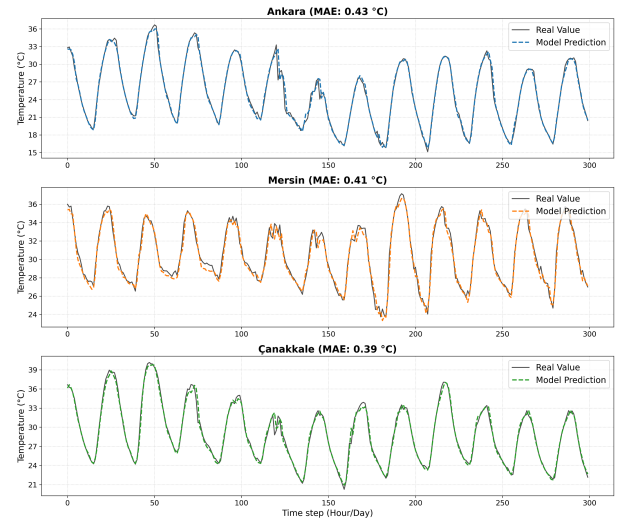
Fig. 3. Temporal temperature predictions for 1-hour forecast horizon.
