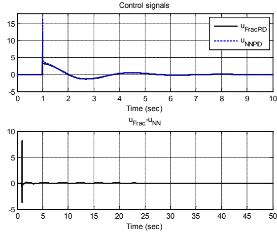
Fig. 6. The control signals generated by the PI^{\lambda}D^{\mu} controller and its neural network based substitute. The bottom row shows the difference in between the two signals.
