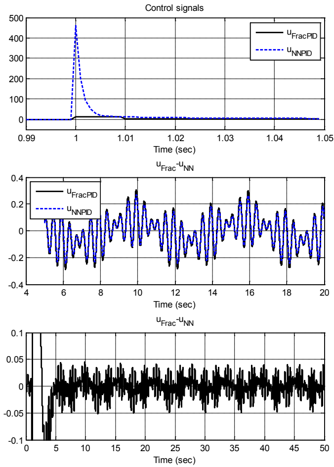
Fig. 8. The control signals generated by the PI^{\lambda}D^{\mu} controller and its neural network based substitute. The top row illustrates the two signals when the step change occurs. The middle row depicts the closeness of the two signals when t > 5 sec., and the bottom row shows the difference in between the two signals.
