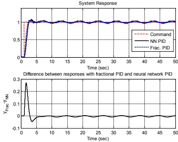
Fig. 7. For the second example, system response and the difference in between the two responses obtained with the PI^\lambda D^\mu controller and its neural network based substitute.
