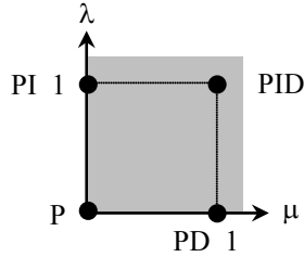
Fig. 2. Continuous values of the differintegration orders \lambda and \mu enables to obtain infinitely many configurations of PI^\lambda D^\mu controller where the variants of the classical PID controller correspond to a subset of the domain.
