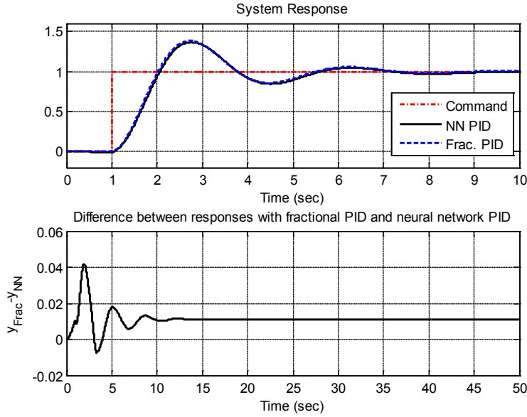
Fig. 5. For the first example, system response and the difference in between the two responses obtained with the PI^\lambda D^\mu controller and its neural network based substitute.
